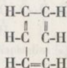
Benzina ( \beta )
