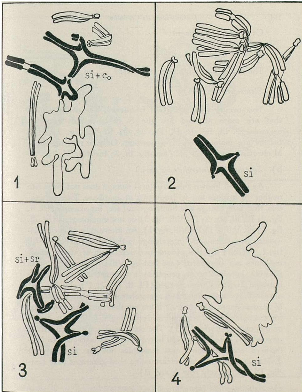
Text-fig. II — 1, Symmetrical interchange between Si - M (?) chromosomes; the nucleolar arm of one M chromosome is broken (see Pl. VII, fig. 3). 2, Symmetrical interchange between two S homologous chromosomes. Only 11 chromosome* can be counted (the squash threw out of cell one of them) (see Pl. VIII, fig. 3). 3, Symmetrical interchange between two S homologous chromosomes, and symmetrical interchange between two S chromosomes, with SR (see Pl. II, fig. 2). 4, Symmetrical interchange between two S non-homologous chromosomes (see Pl. II, fig. 3).
