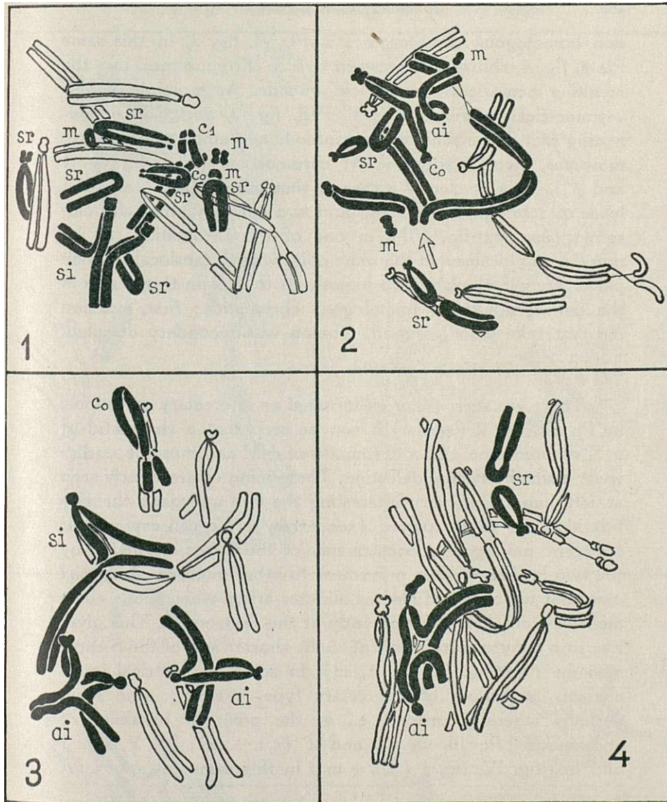
Text-fig. III — 1, Symmetrical interchange between two S chromosomes; breakage in 5 S chromosomes followed by SR; two minutes (m) originated by breakage at the centromere (see Pl. IV, fig. 1). 2, Si-S asymmetrical interchange (ai); breakage in 3 S chromosomes followed by SR; simulated pairing of non-homologous chromatids (arrow) (see Pl. IV, fig. 2). 3, Breakage close to the centromere of the M chromosome giving rise to the Co acentric fragment, followed by interchange (read ai instead of si) with an S chromosome; two S-S asymmetrical interchanges (ai) (see Pl. IV, fig. 3). 4. SR in a S chromosome; asymmetrical interchange between Si-S chromosomes (ai) (see Pl. IV, fig. 4). X 2.200.
