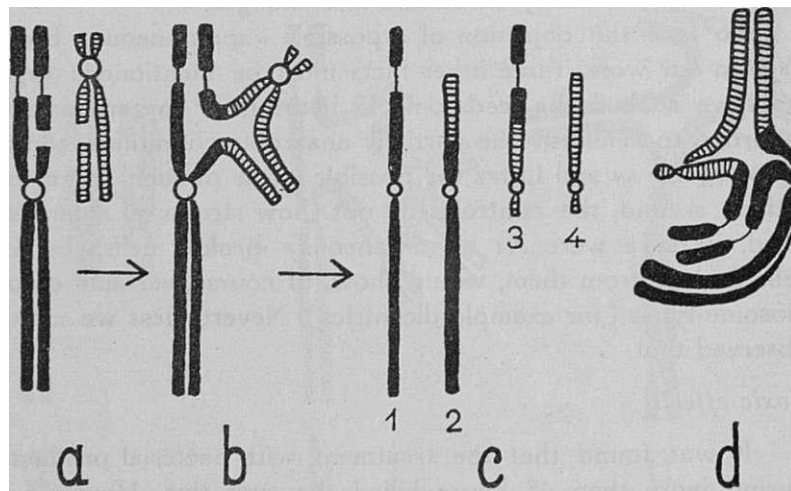
Text-fig. VIII — Diagram showing how new chromosome types arise by symmetrical interchange between M - S chromosomes:
