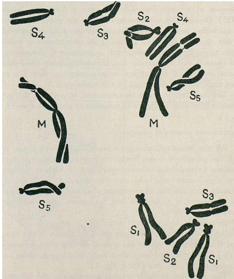
Text-fig. I — The 12 chromosomes of Vicia faba (see also Plate I, fig. 1 ). X 2.700.
